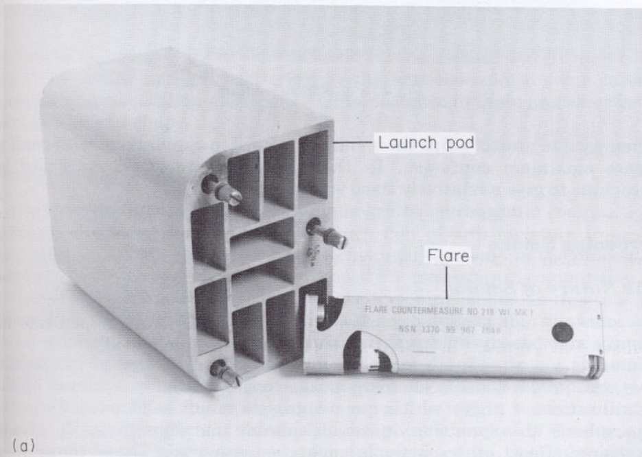
FIG. 7.7a Launch pod
