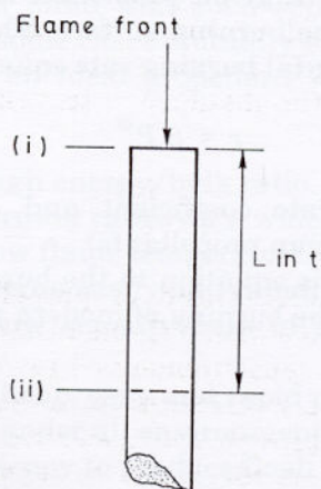
FIG. 5.3 Propellant strand
