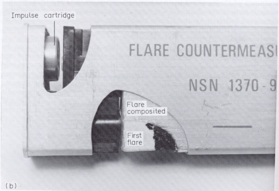
FIG. 7.7b '218' infra-red flare
