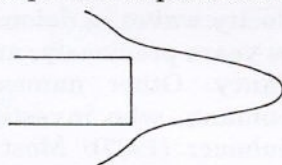
FIG. 2.11 Shockwave from a plane-ended charge
