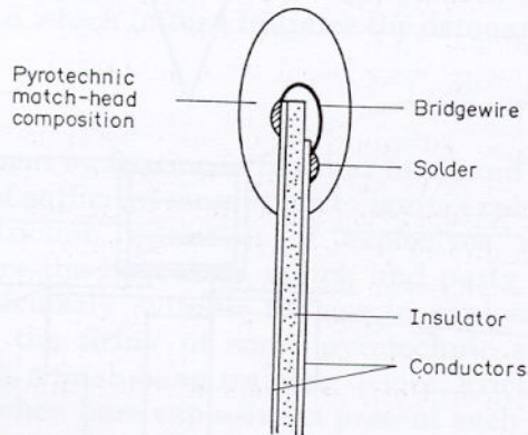
FIG. 4.9 Bridgewire initiation
