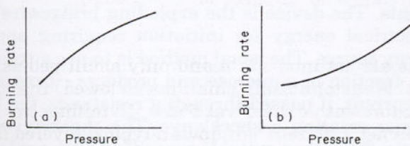
FIG. 4.12 Burning rate versus pressure
